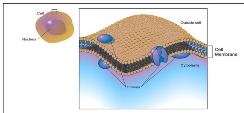
Fig 1: Plasma membrane
