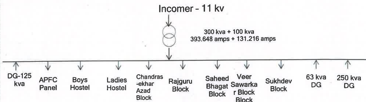
FIGURE 4: SINGLE LINE DIAGRAM – ELECTRICAL
